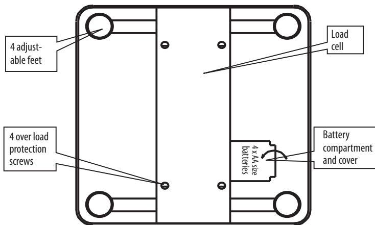
Fig 1: Bottom view of the scale
